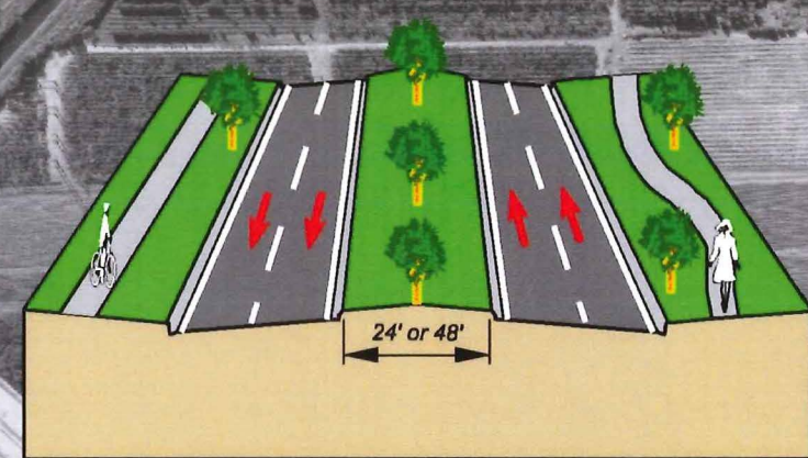
4-Lane Typical Section See Appendix For Details
