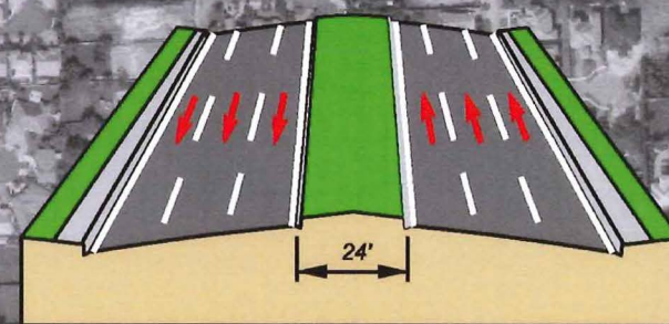
6-Lane Typical Section
