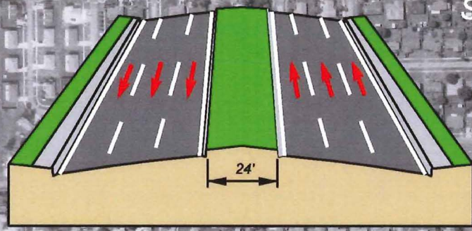
6-Lane Typical Section
