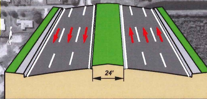
6-Lane Typical Section See Appendix For Details
