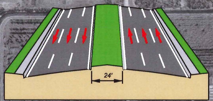
6-Lane Typical Section
