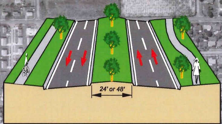
4-Lane Typical Section See Appendix For Details
