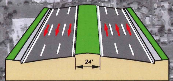
6-Lane Typical Section See Appendix For Details
