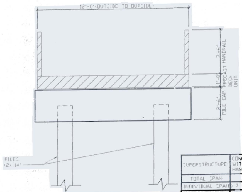
SECTION "A-A" SCALE 1"=30'
