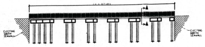
ELEVATION LOOKING WEST SCALE 1"=300'
