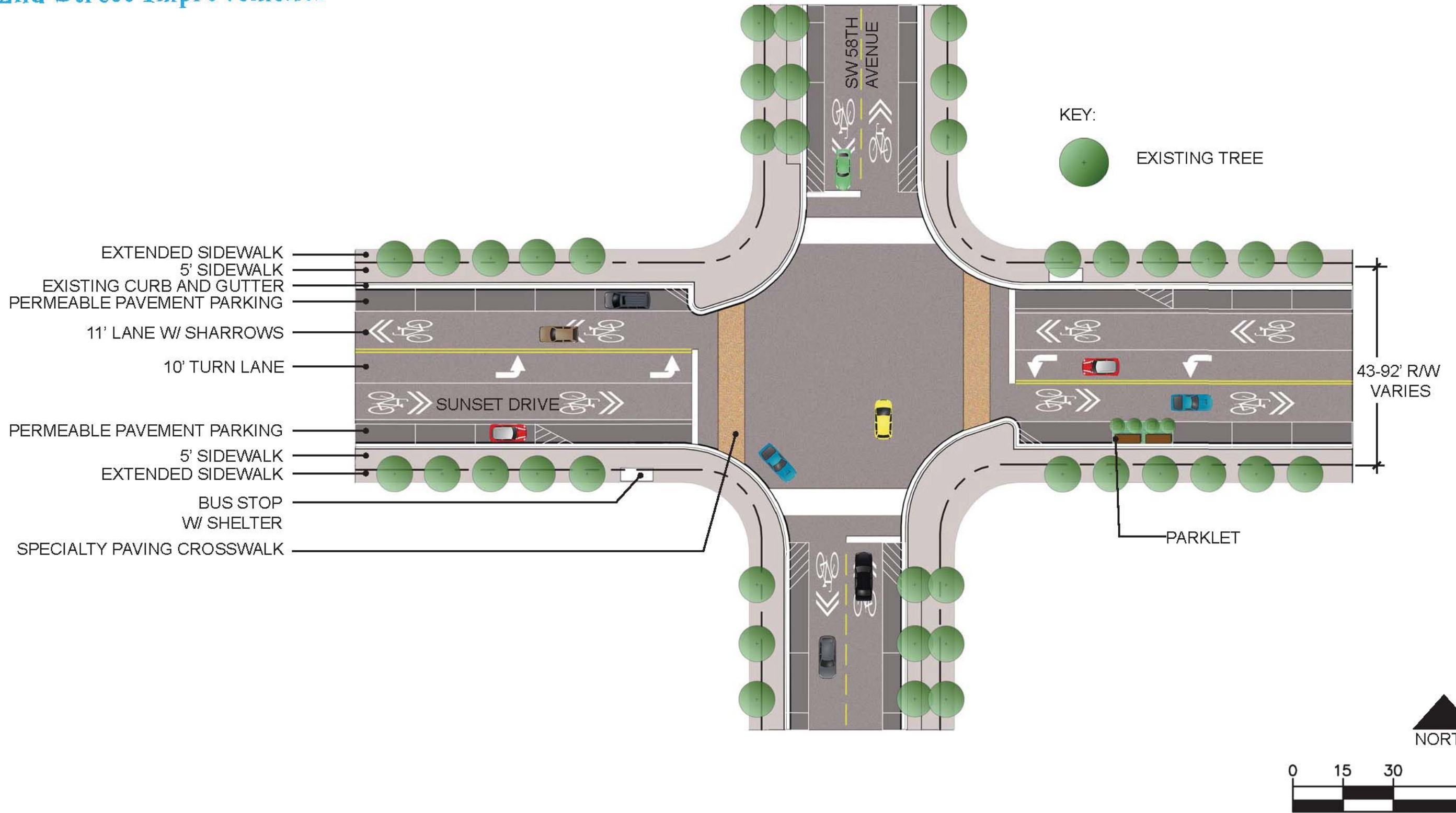
Figure 22: SW 72nd Street Improvements
