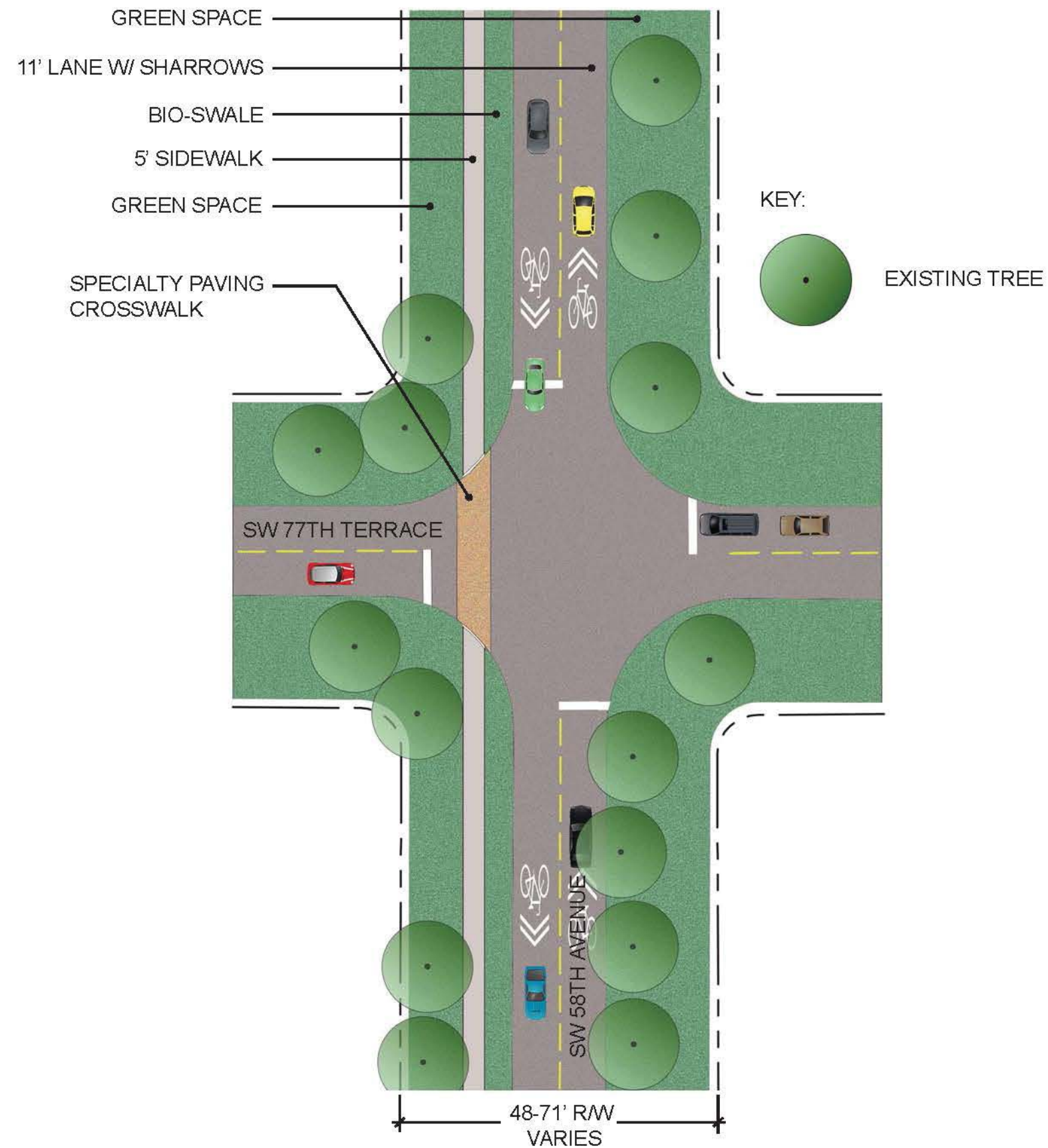
Figure 28: SW 58th Avenue Improvements
