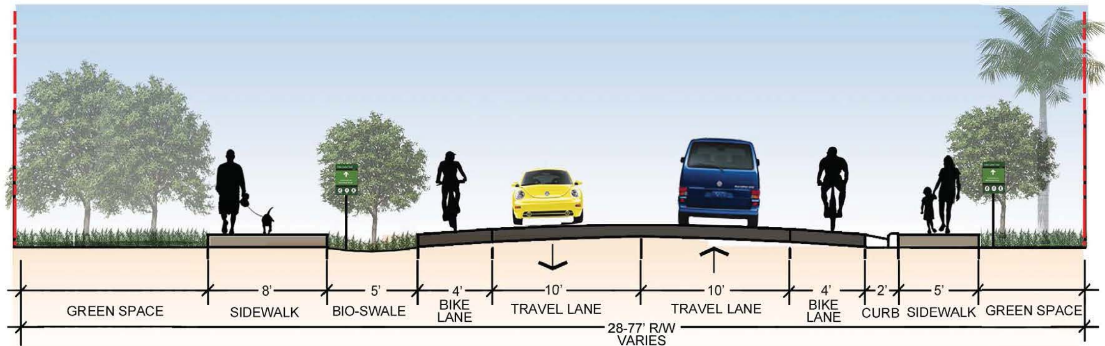
SW 62ND AVENUE PROPOSED (LOOKING NORTH)
