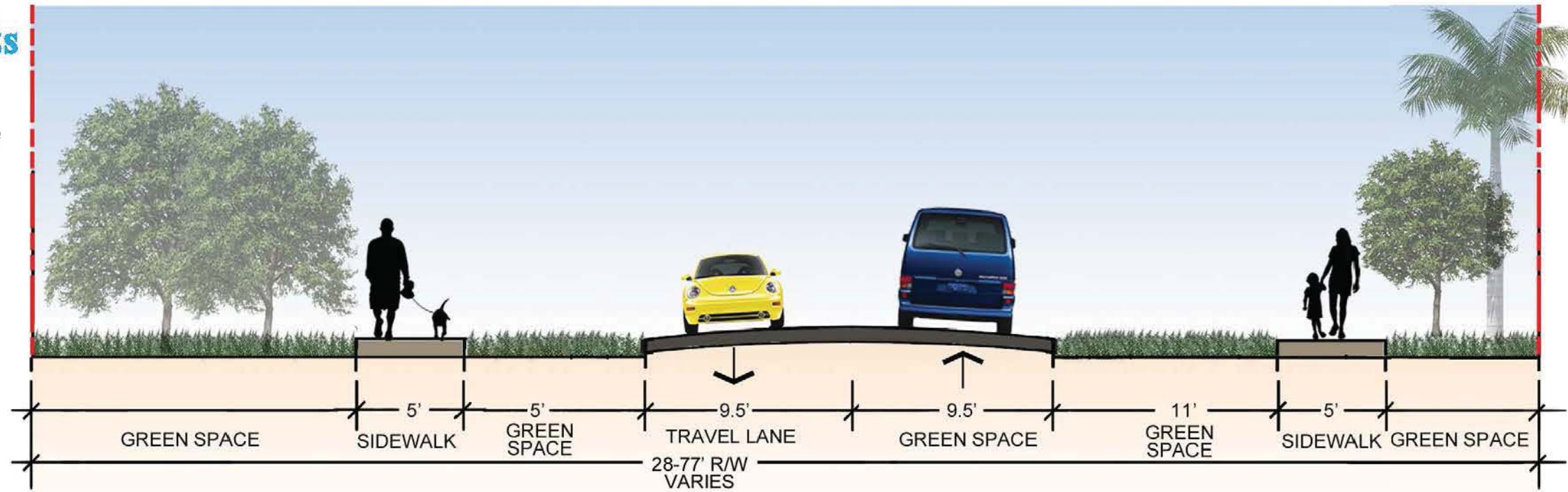
SW 62ND AVENUE EXISTING (LOOKING NORTH)
