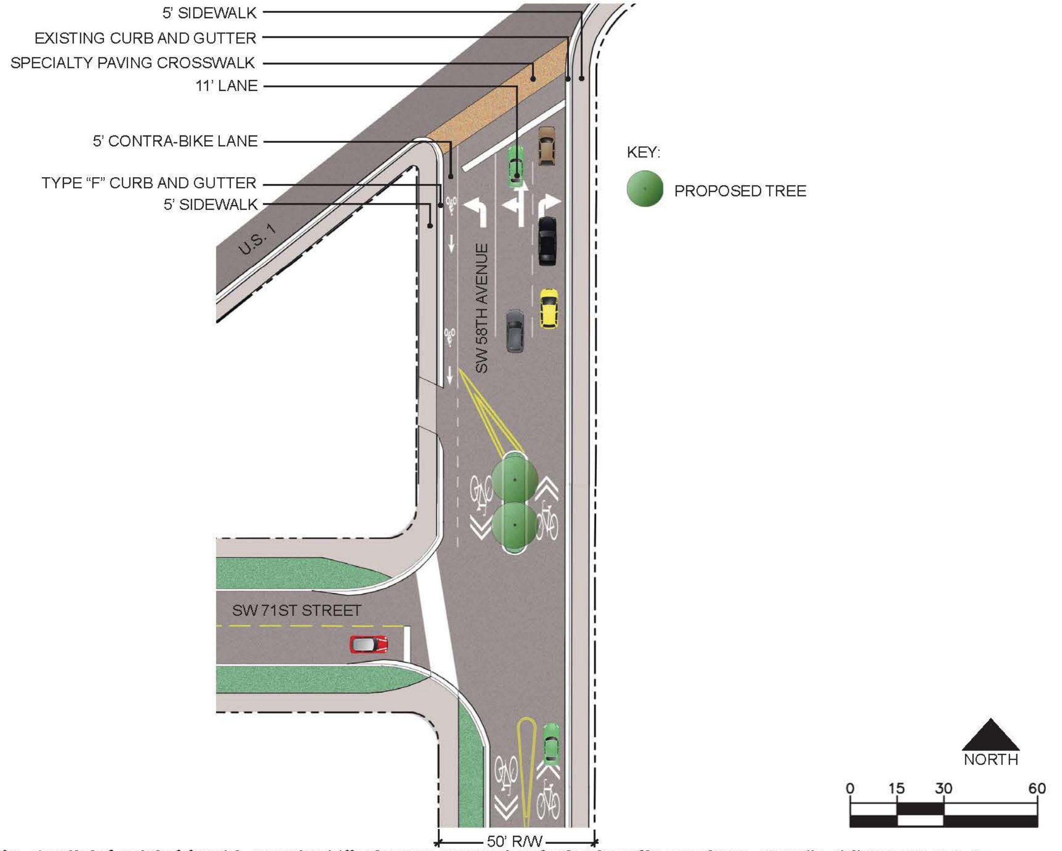
Figure 26: SW 58th Avenue Improvements
