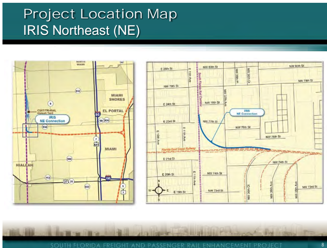
Figure 2.7 Northeast IRIS Connection Between CSX and FEC
