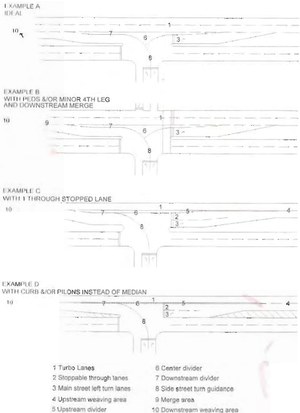
FIGURE 1 TYPICAL TURBOLANE INTERSECTION DESIGNS
